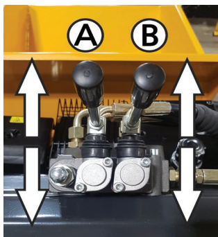
lever control valve (6) for raising and lowering the tipping trough (A) or the self-loading shovel (B)
